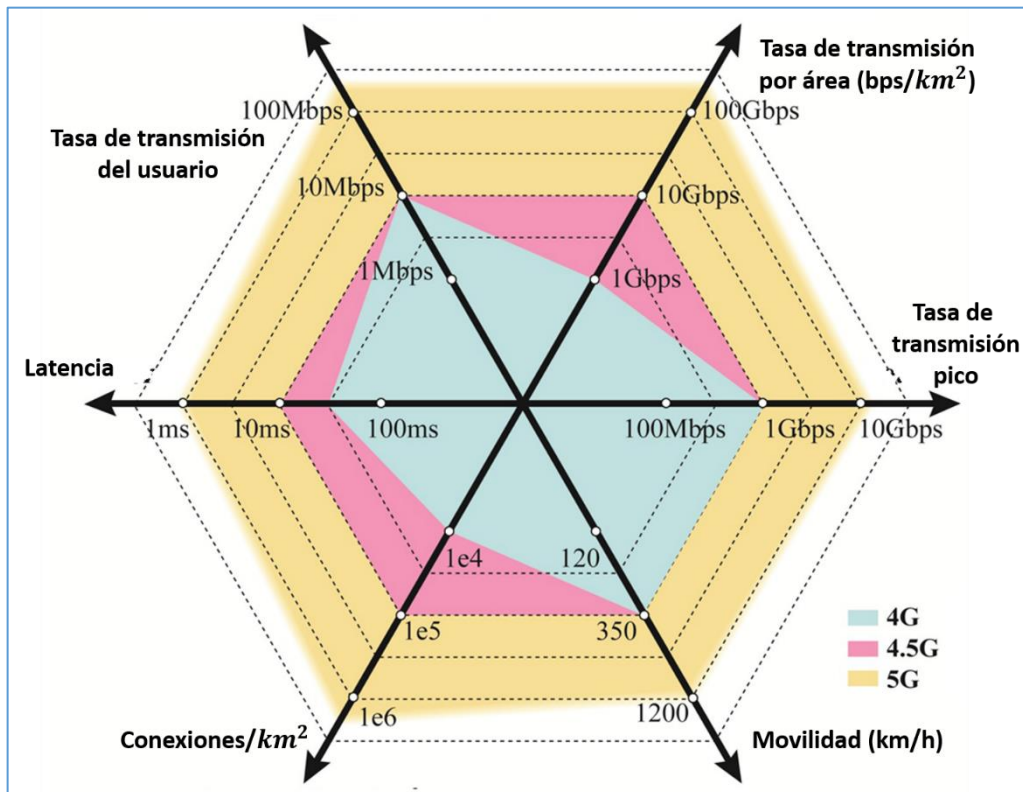
Gráfica 1. 5G versus 4G. [Osseiran (2016)].
